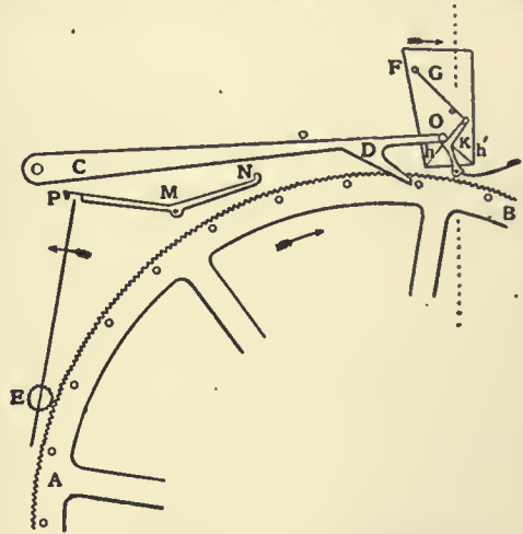
FIG. 21.—Chronometer Spring Remontoire.
